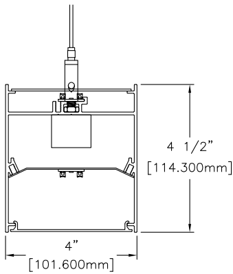
Indirect clear acrylic (CA) lens w/Direct flush lens (FL) shown. See page 6 for other lens details.
